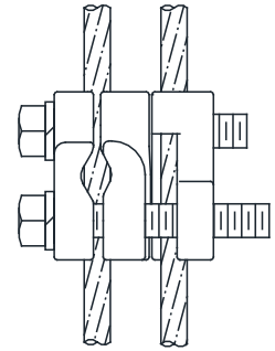
Parallel Bolted
