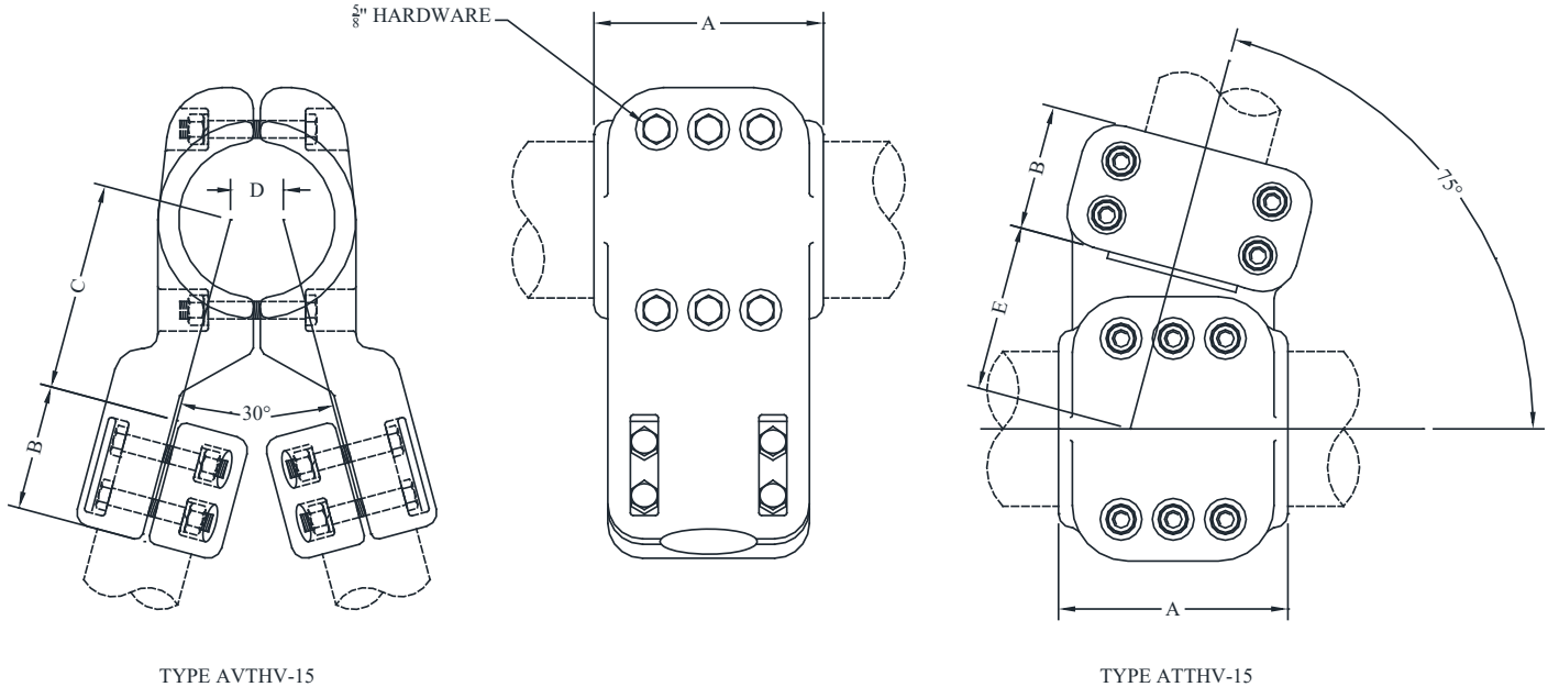
TYPE AVTHV-15
