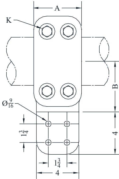
TYPE ATFHV
